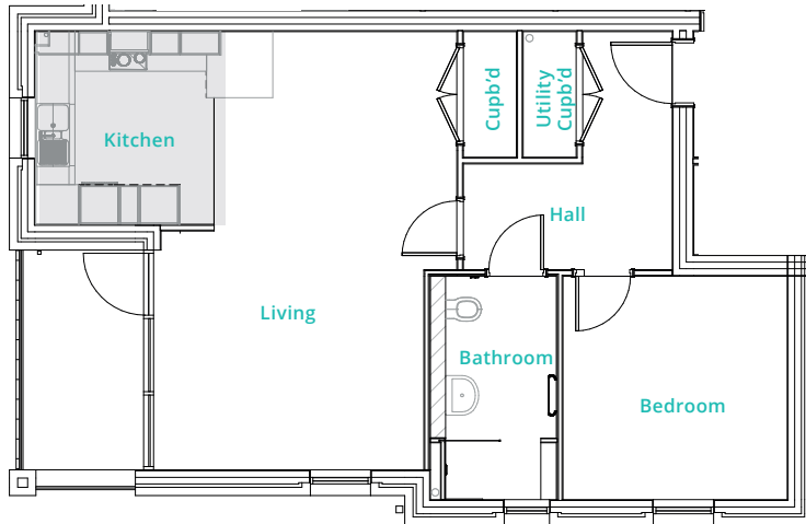
Typical Layout
